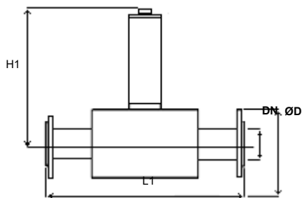
flange design
