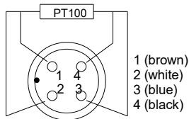
M12 plug (only PT100)
