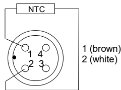
M12 plug (only NTC)
